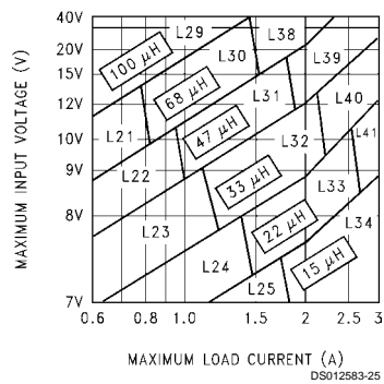
FIGURE 5. LM2596-5.0
