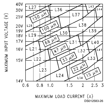
FIGURE 6. LM2596-12
