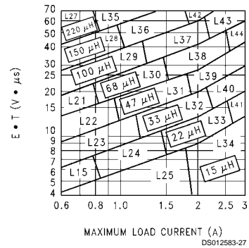
FIGURE 7. LM2596-ADJ
