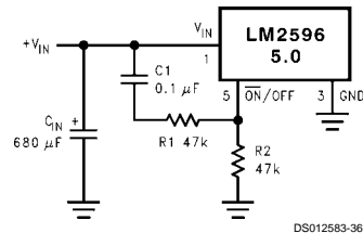
FIGURE 21. Delayed Startup
