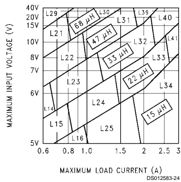
FIGURE 4. LM2596-3.3
